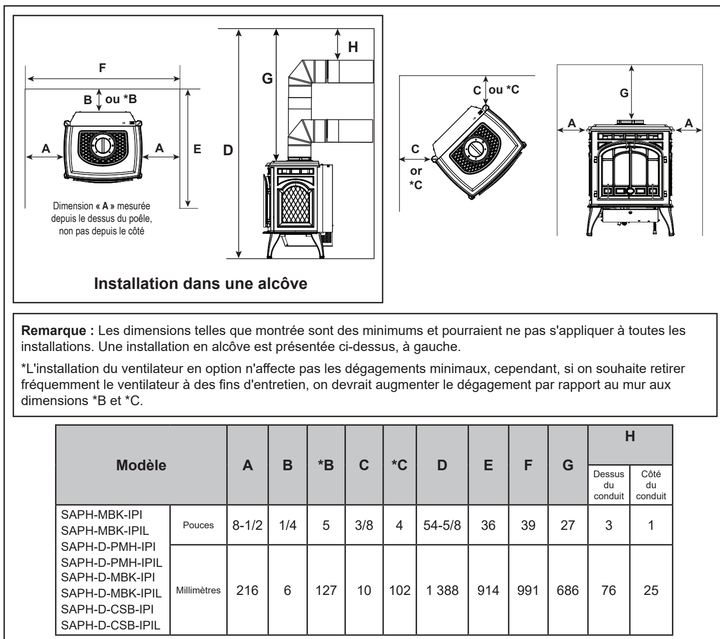
Figure 3.2 Emplacements du foyer
