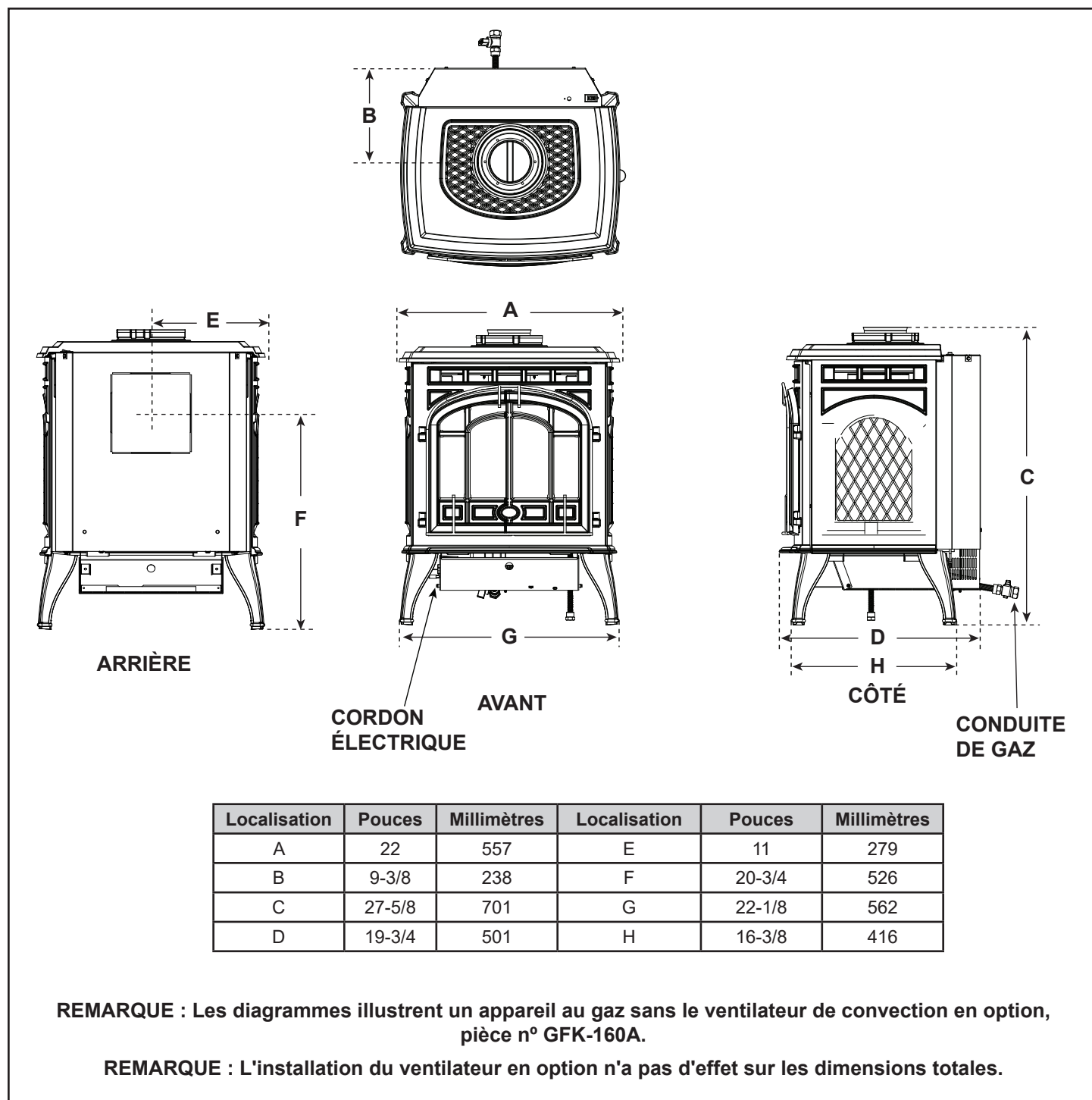
Figure 3.1 Dimensions du foyer
