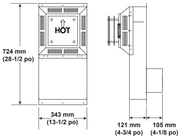
SLK-SNKD Snorkel Termination Cap
