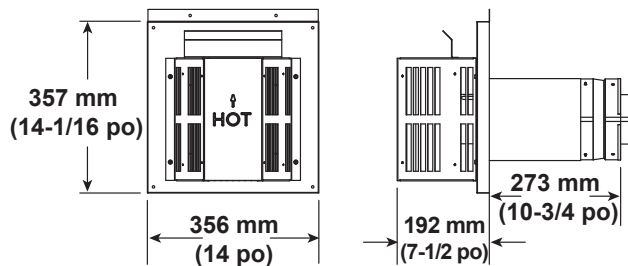
Kit de terminal horizontal SLP-FLEX-TRAP
