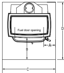
Standard Dimensions
