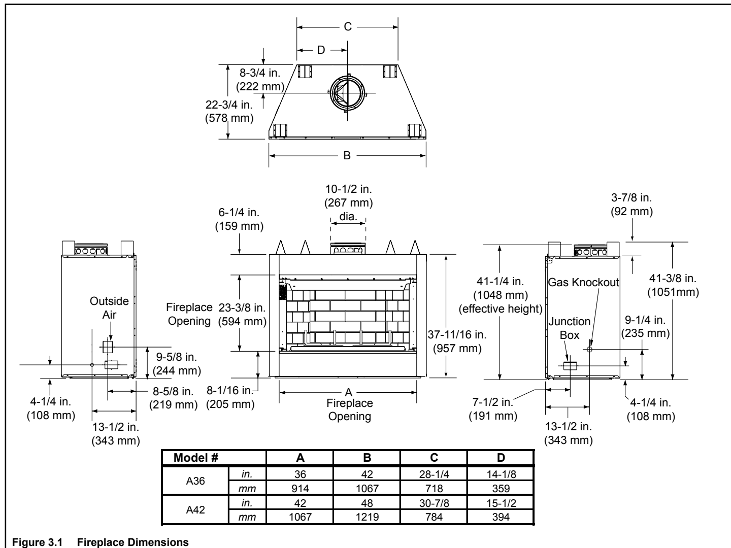
Figure 3.1 Fireplace Dimensions
