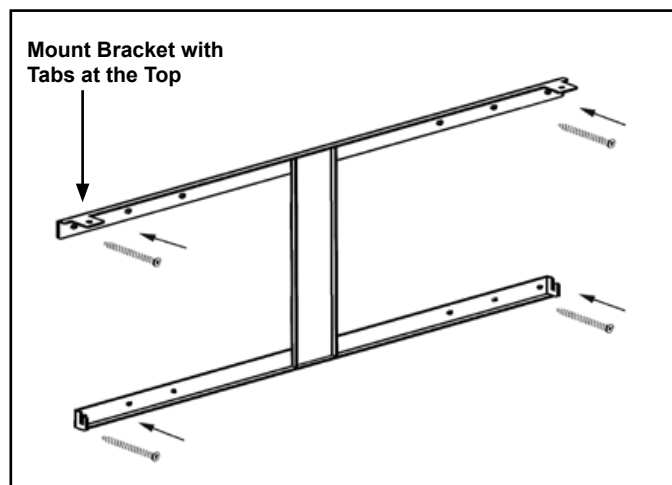
Figure 4.3 Bracket Attachment
