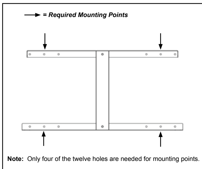
Figure 4.1 Mounting Bracket
