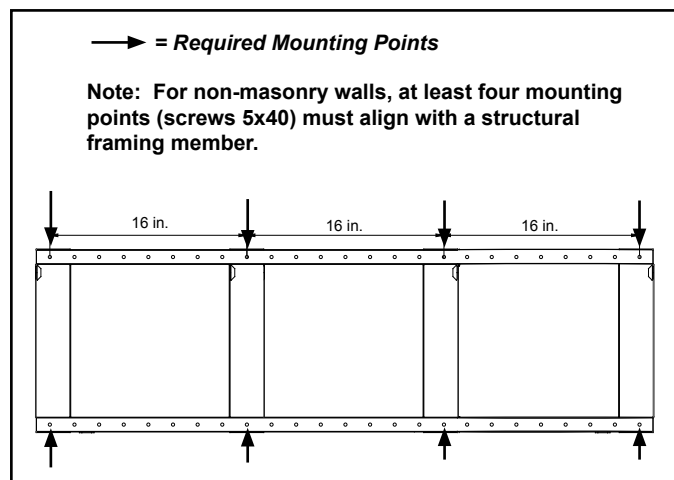
Figure 4.2 Mounting Bracket
