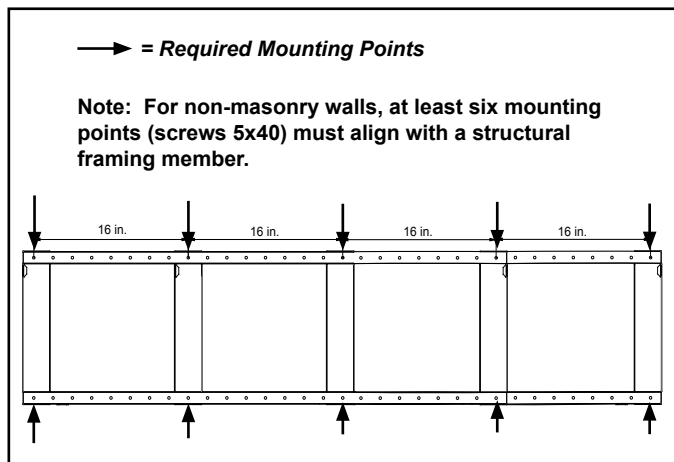
Figure 4.3 Mounting Bracket
