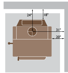
Floor protection: 32-5/8"W x 51-7/16"D
