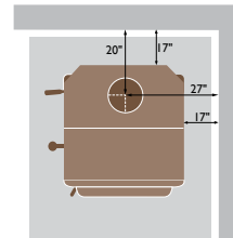
Floor protection: 32-1/2"W x 50-7/16"D
