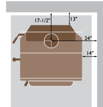
Floor protection: 32-1/2"W x 48"D
