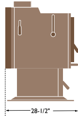
Side View/Pedestal
