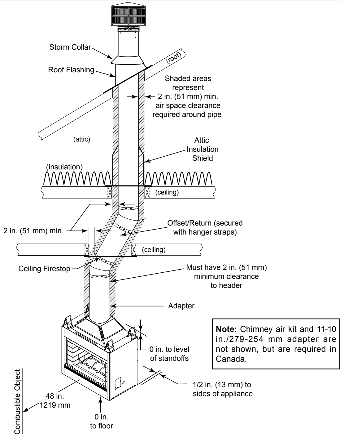
Figure 3.2 Clearances to Combustible Materials
