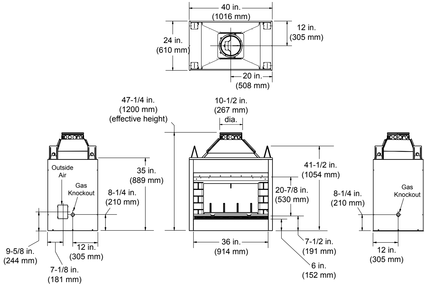
Figure 3.1 Fireplace Dimensions
