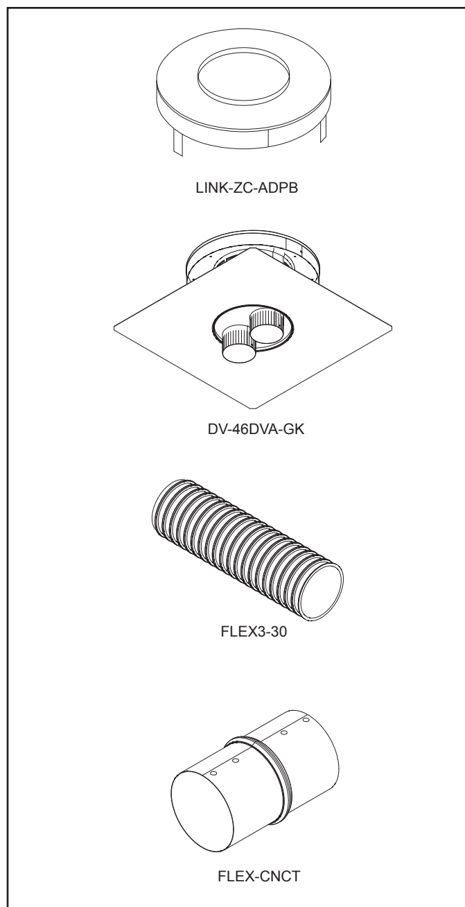
Figure 14.5 Direct Vent Flex Liner Accessory Kits
